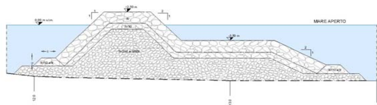
TYPICAL CROSS SECTIONS
