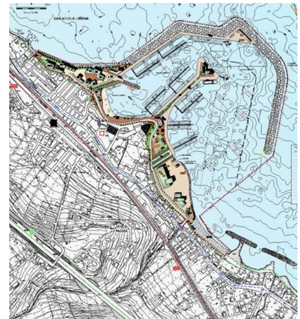
PRELIMINARY DESIGN
