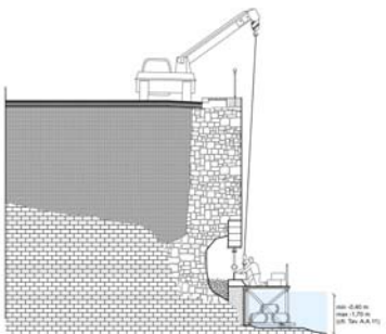
RESTORE OF VOLUMES DETACHED AND MORTAR JOINTS
