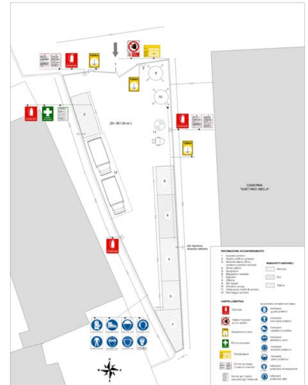
WORKSITE PLAN
