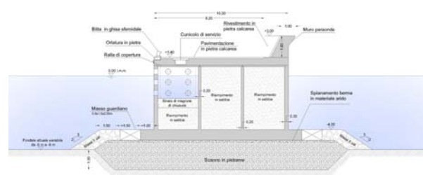
TYPICAL CROSS SECTIONS
