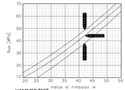
HAMMER TEST
