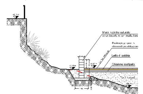
NEW COASTLINE DEFENSE WORKS: PLAIN AND TYPICAL CROSS SECTIONS
