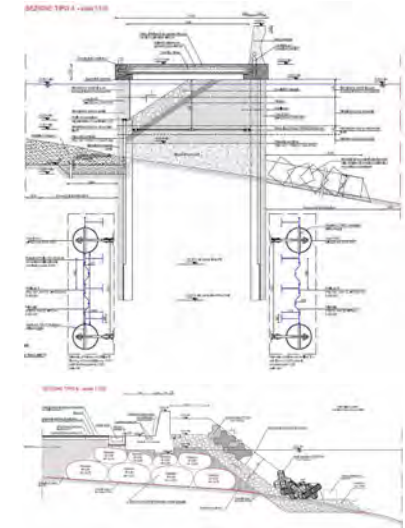
TYPICAL CROSS SECTIONS
