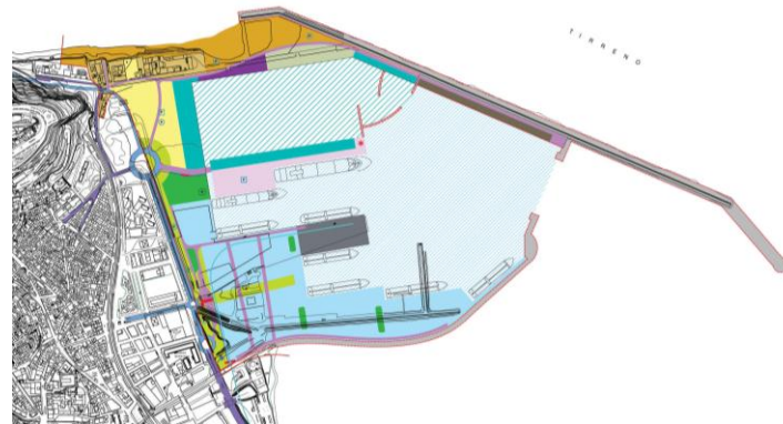
LOGISTIC PLAN
