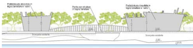
LONGITUDINAL PROFILE 'S' FRAME OF FACILITIES AREA
